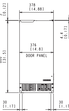
FRONT DIMENSIONS (ADA compliant unit)
